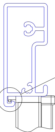
DETAIL A
