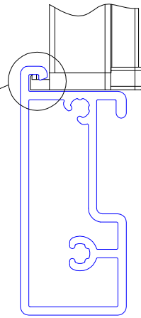
DETAIL C
