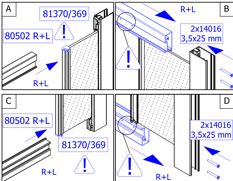
DETAIL A
